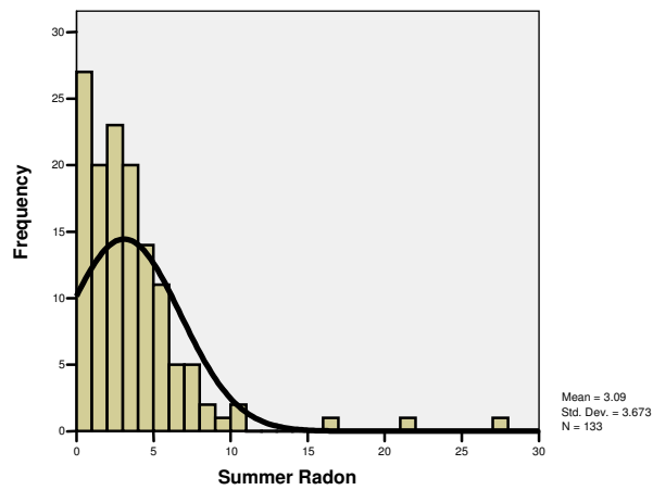
Figure 7. Histogram of Summer Indoor Radon in the Pope's Head Formation Homes
