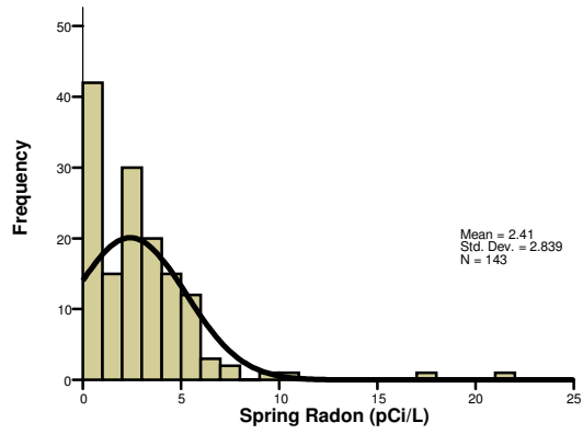
Figure 2. Histogram of Spring Indoor Radon in the Sykesville Formation Homes
