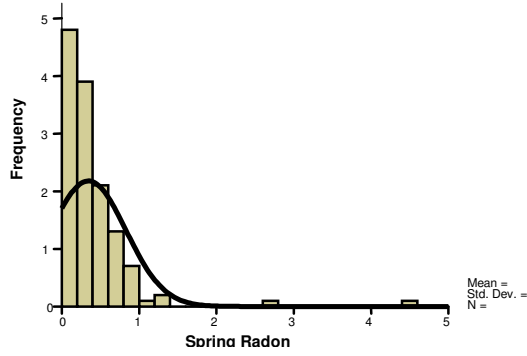
Figure 6. Histogram of Spring Indoor Radon in the Pope's Head Formation Homes
