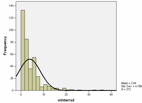
Figure 9. Histogram of Winter Indoor Radon in the Mather Gorge Formation Homes
