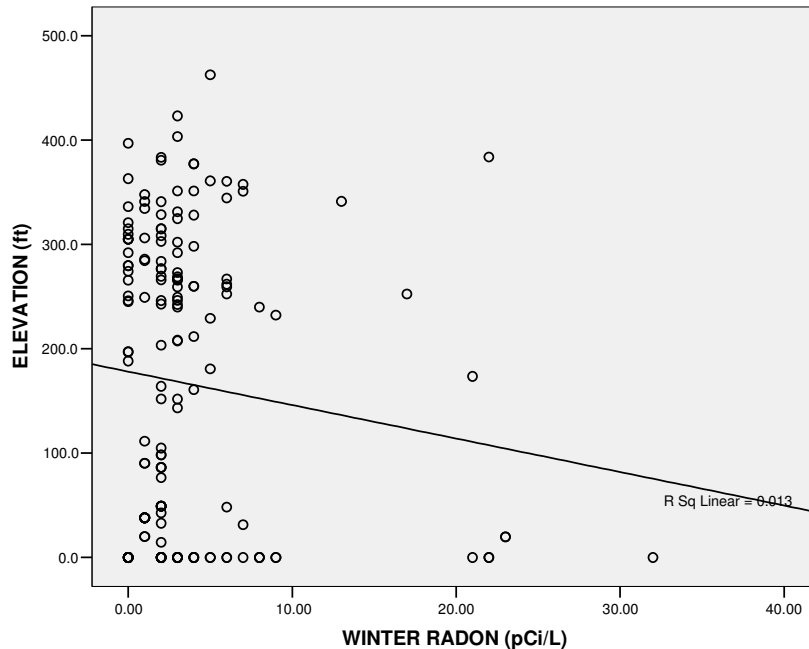
Figure 14. Scatter Plot of Elevation and Winter Indoor Radon Measurements
