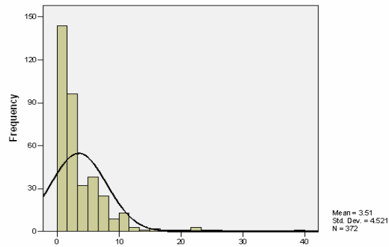
Figure 10. Histogram of Spring Indoor Radon in the Mather Gorge Formation Homes
