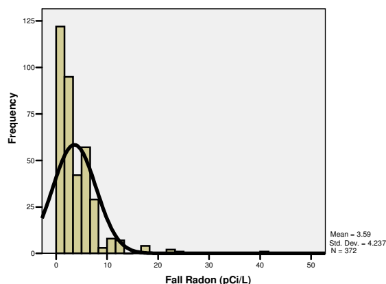
Figure 12. Histogram of Fall Indoor Radon in the Mather Gorge Formation Homes
