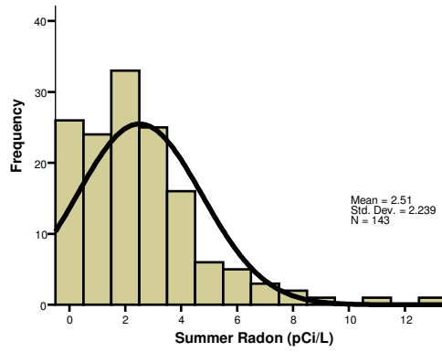
Figure 3. Histogram of Summer Indoor Radon in the Sykesville Formation Homes
