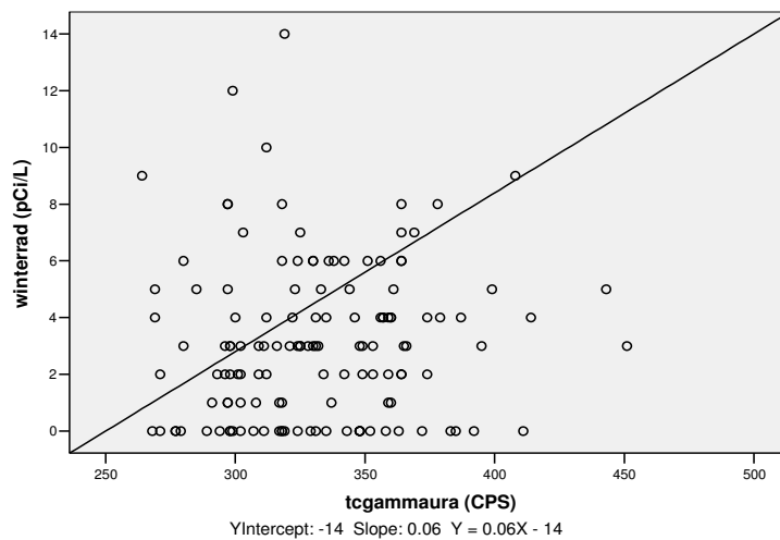
Scatter Plot of Indoor Winter Radon vs. Aeroradioactivity for Pope's Head Formation Homes
