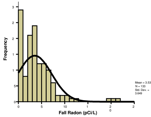
Figure 8. Histogram of Fall Indoor Radon in the Pope's Head Formation Homes
