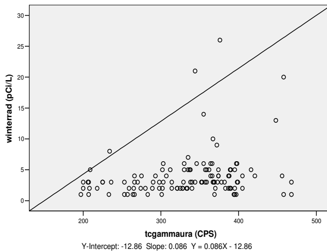
Scatter Plot of Indoor Winter Radon vs. Aeroradioactivity for Sykesville Formation Homes
