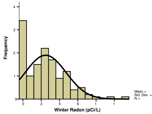
Figure 5. Histogram of Winter Indoor Radon in the Pope's Head Formation Homes
