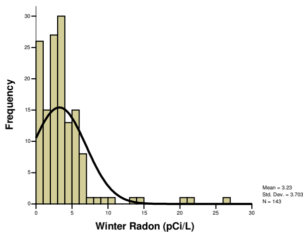
Figure 1. Histogram of Winter Indoor Radon in the Sykesville Formation Homes
