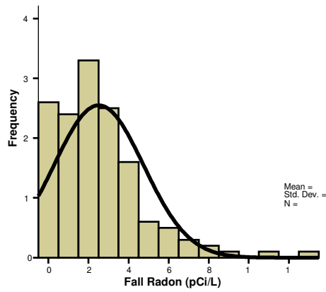
Figure 4. Histogram of Fall Indoor Radon in the Sykesville Formation Homes
