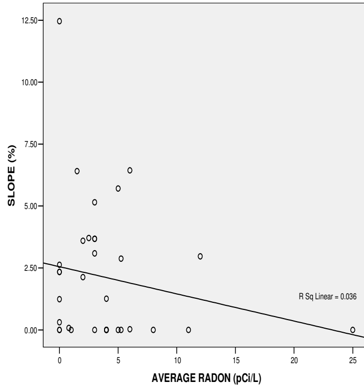
Figure 13. Scatter Plot of Slope and Winter Indoor Radon Measurements
