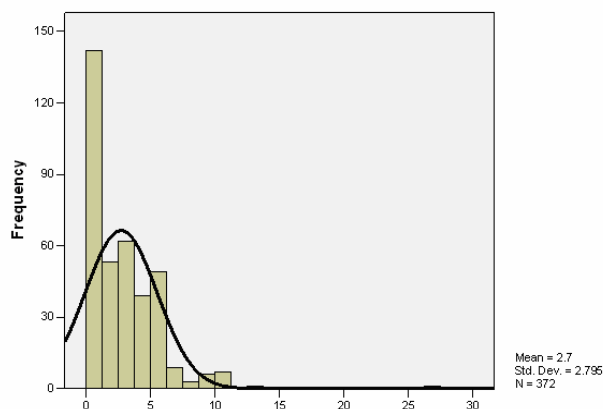
Figure 11. Histogram of Summer Indoor Radon in the Mather Gorge Formation Homes
