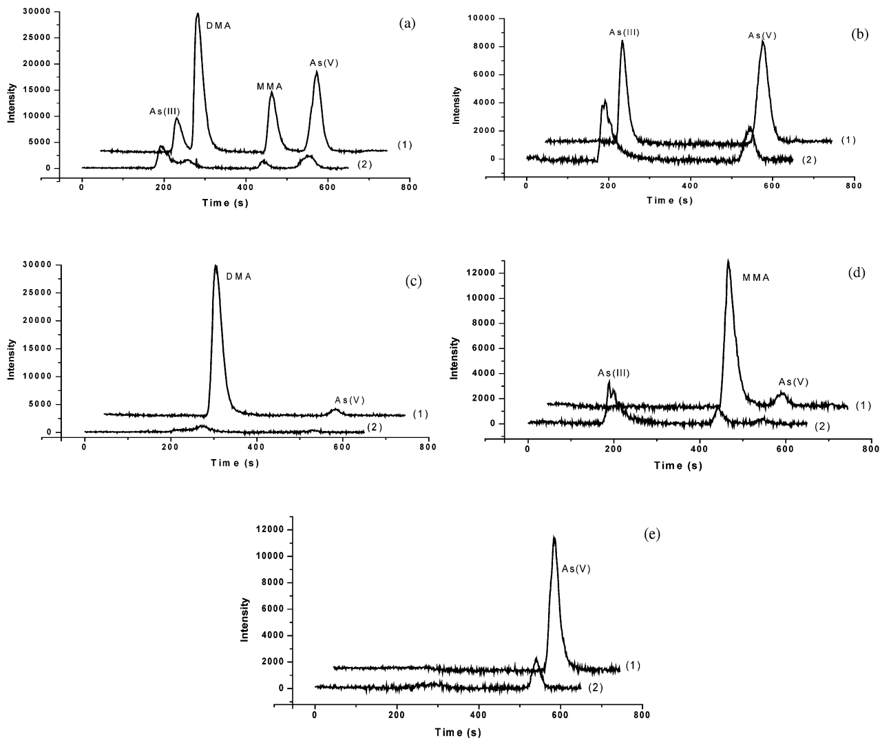
Fig. 4 Chromatograms for arsenic speciation by HPLC-HG-ICP-OES of sequential extracts of (a) mixed species-soil, (b) As(III)-soil, (c) DMA-soil, (d) MMA-soil, and (e) As(V)-soil; 1. 0.10 mol l -1 H 3 PO 4 ; 2. 0.10 mol l -1 NaOH.
