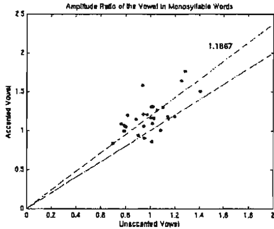
a. Amplitude Ratio in Monosyllable Data
