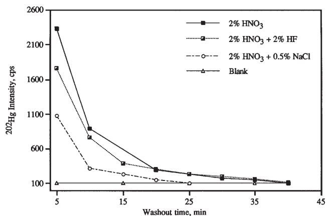
Fig. 1 Effect of various solutions on residual Hg washout as a function of time
