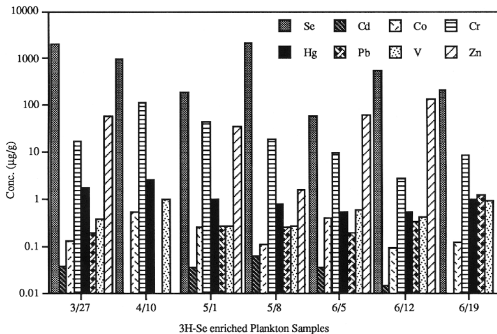
Fig.3 The effect of Se on the planktonic uptake of Cd, Co, Cr, Hg, Pb, V and Zn (3H Se-enriched plankton samples)
