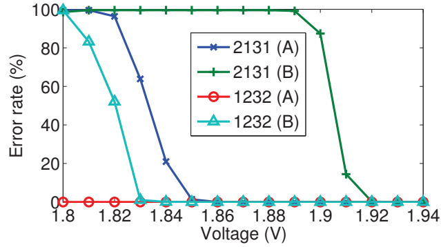
Figure 4.4. Flash write error rates decrease as voltage increases. This trend holds for all the chips we tested, though error rates differ even between chips of the same model.
