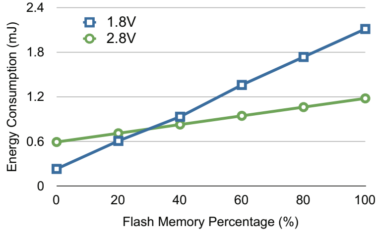
Figure 4.14. Energy consumption of TI MSP430 microcontroller for different workloads of flash memory. The experimental results verify the calculation of finding the cross-over point at which in-place writes are competitive over normal flash writes. The cross-over point is where the time spent on computation is at least four times greater than the time spent on flash writes.
