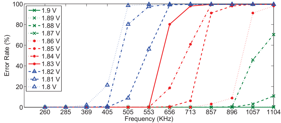
Figure 4.15. Error rate declines when the writes are performed at a lower frequency. For a voltage level as low as 1.8 V, the average error rate is zero when the writes are performed at 260 KHz while for 1.9 V (still well below the recommended voltage), the average error rate is zero even if the memory is used at full speed.
