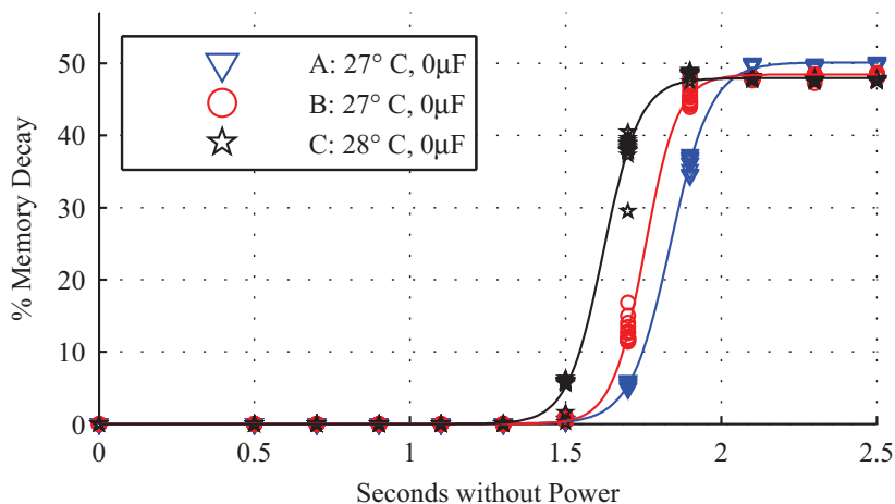
Figure 5.11. Decay versus time in 3 different instances of the MSP430F2131 microcontroller at similar temperatures. The durations of Stage 1 and Stage 2 decay match closely across instances.
