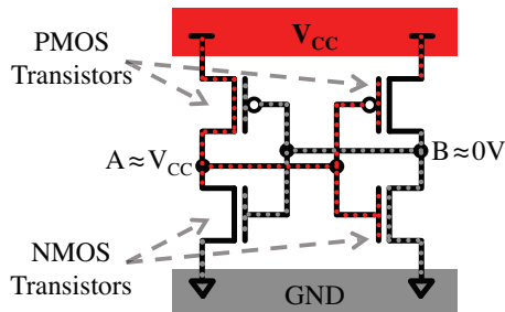
Figure 5.13. The state-holding portion of an SRAM cell consists of two cross-coupled inverters tied to the chip's power and ground nodes.
