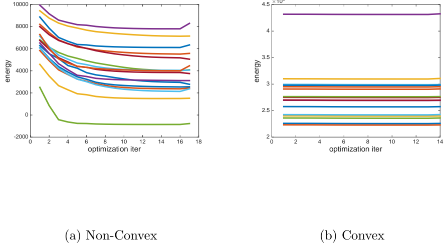
Figure 8.7: Test-time energy minimization for SPENs trained with and without the restriction that they are input-convex. As before, we append the energy of the ground truth as the rightmost point in each curve. In (a), we find that energy minimization for non-convex energies sometimes returns a value greater than the energy of the ground truth. In (b), this never occurs. However, the energy barely changes between the beginning and the end.
