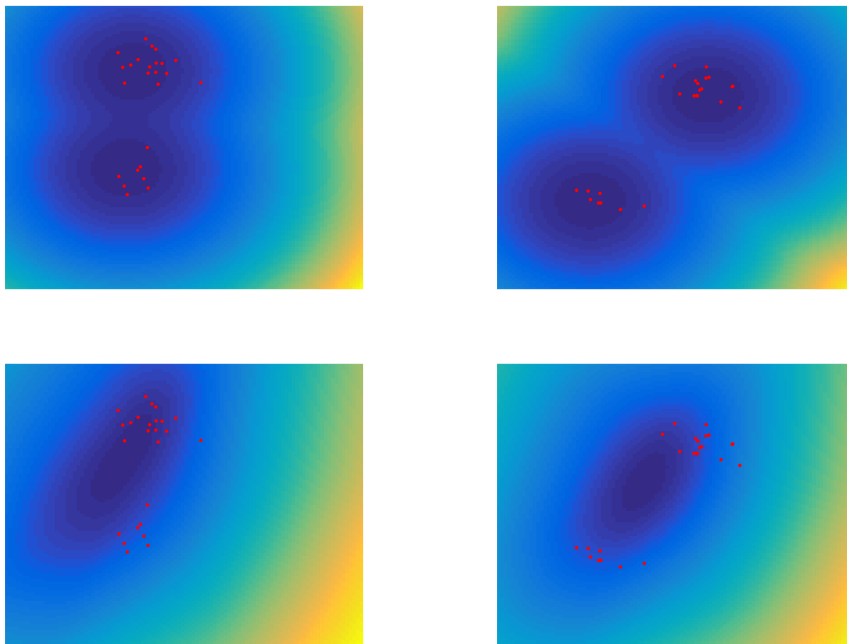
Figure 11.2: Learned energy functions from stochastic MLE training. Each column uses a different value of x , from which we draw multiple samples of y from a conditional GMM. Top row: GMM energy function. Bottom row: MLP energy function.
