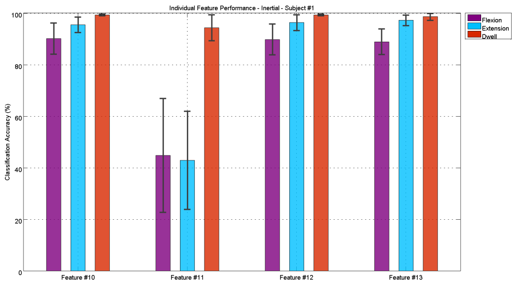
Figure 4.4: Classification performance of individual inertial features with 1-Classifer LDA; Subject #1.
