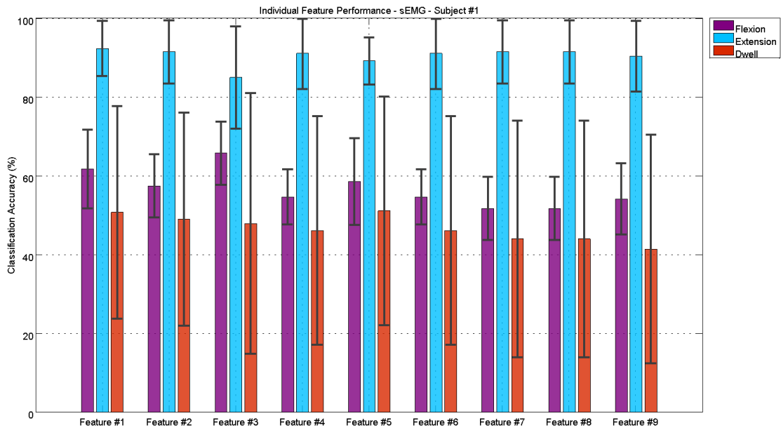
Figure 4.3: Classification performance of individual sEMG features with 1-Classifer LDA; Subject #1.
