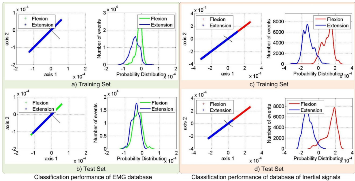
Figure B.1: Two-class classification performance of separate sEMG signals and inertial signals.
