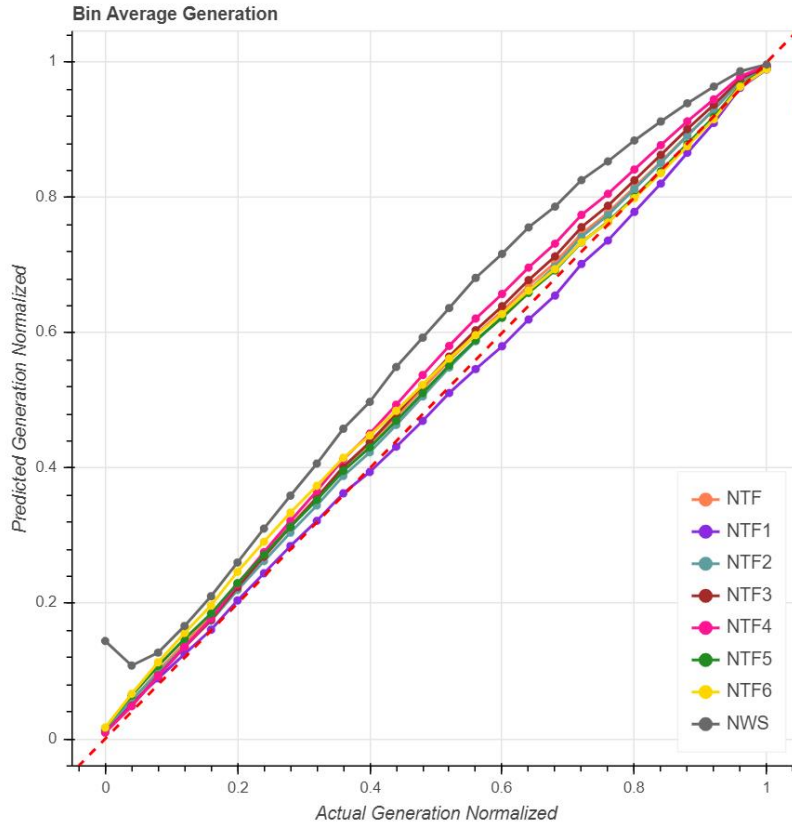
Figure 8: Bin Average Generation for all NTFs
