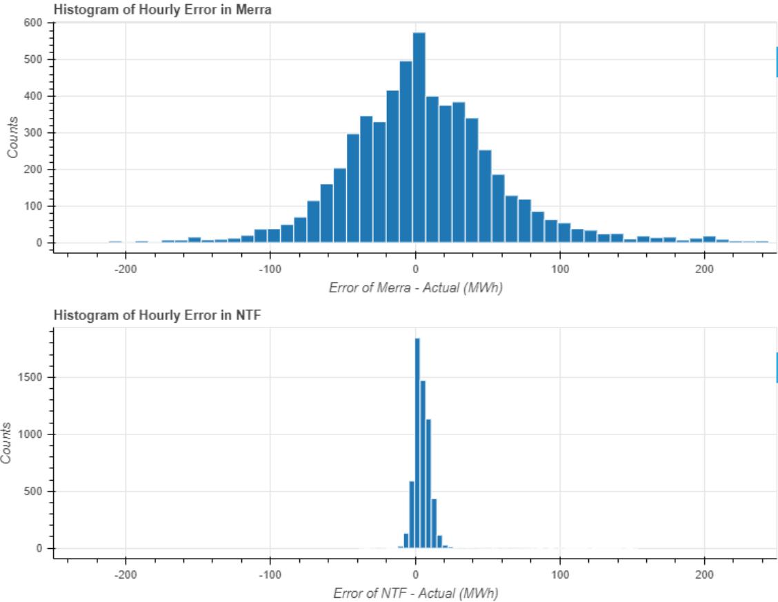
Figure 18: Error in PG Histogram
