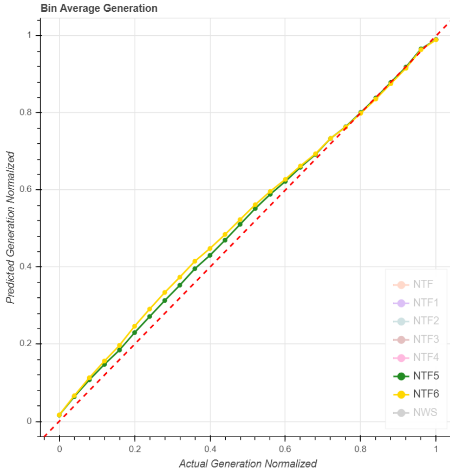
Figure 12: Bin Average Generation mast/turbine pair comparison 2
