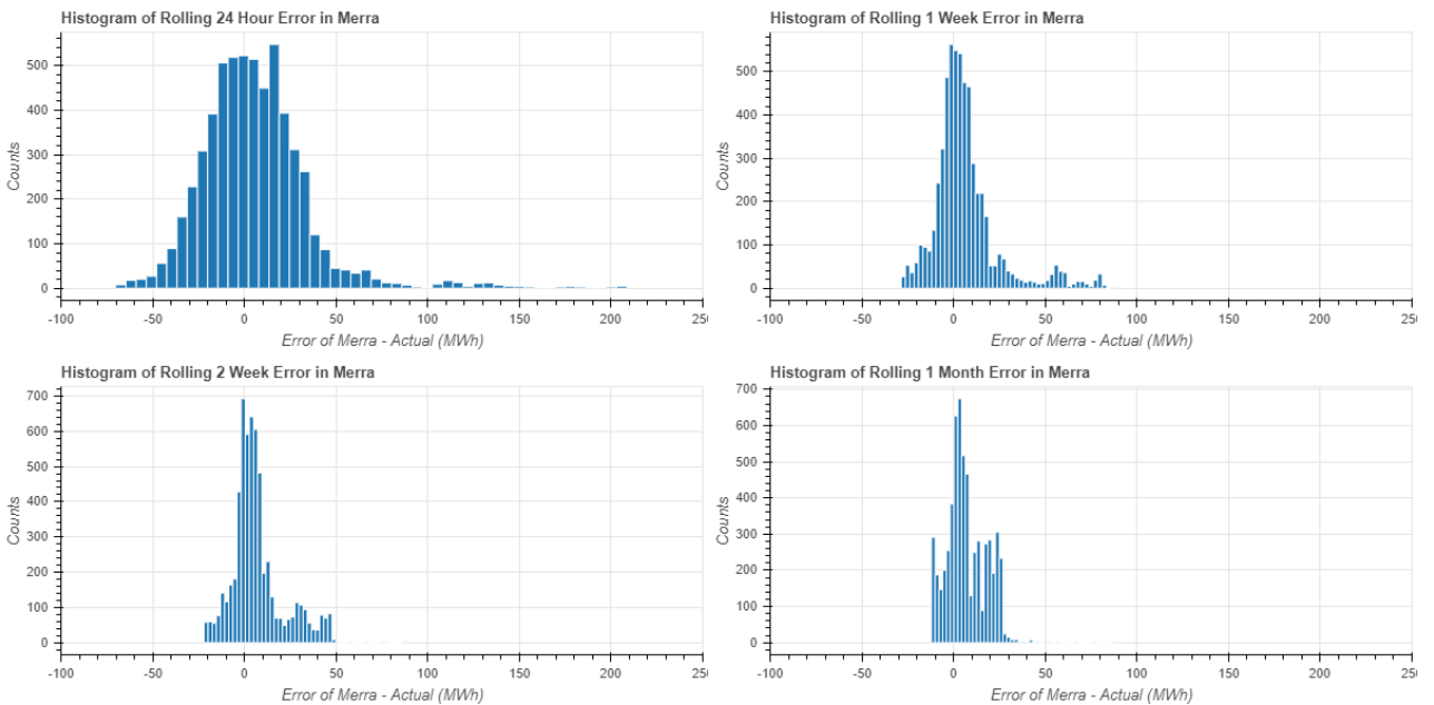
Figure 23: MERRA-2 PG Rolling Average Histograms
