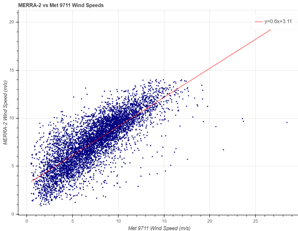
Figure 14: MERRA-2 vs Met 9711 Wind Speeds
