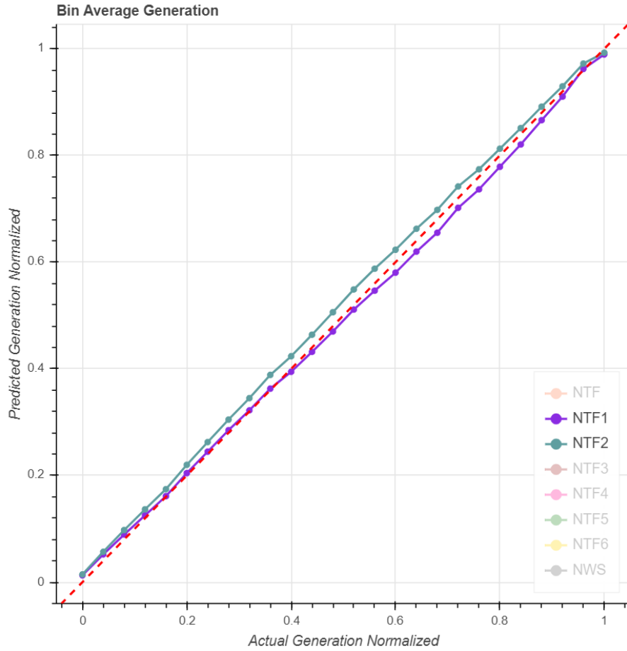
Figure 11: Bin Average Generation mast/turbine pair comparison 1
