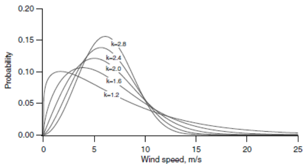
Figure 2: Weibull probability density function for \bar{U} = 6 m/s [2]
