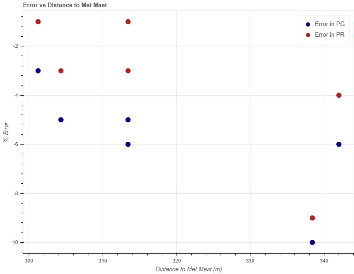
Figure 13: Distance to Met Mast vs Error
