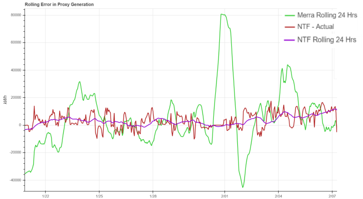
Figure 21: NTF vs MERRA Rolling Average Error in Generation
