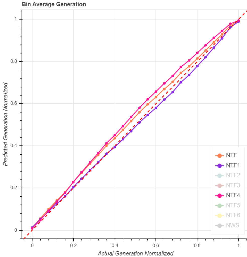
Figure 10: Bin Average Generation NTF method range
