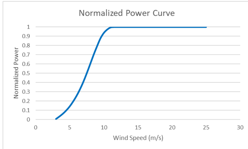
Figure 7: Manufacturer power curve
