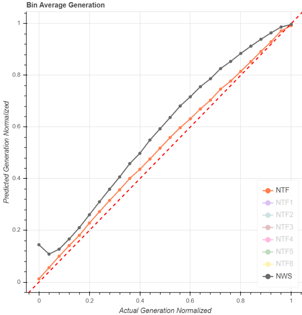
Figure 9: Bin Average Generation for site wide NTF and NWS
