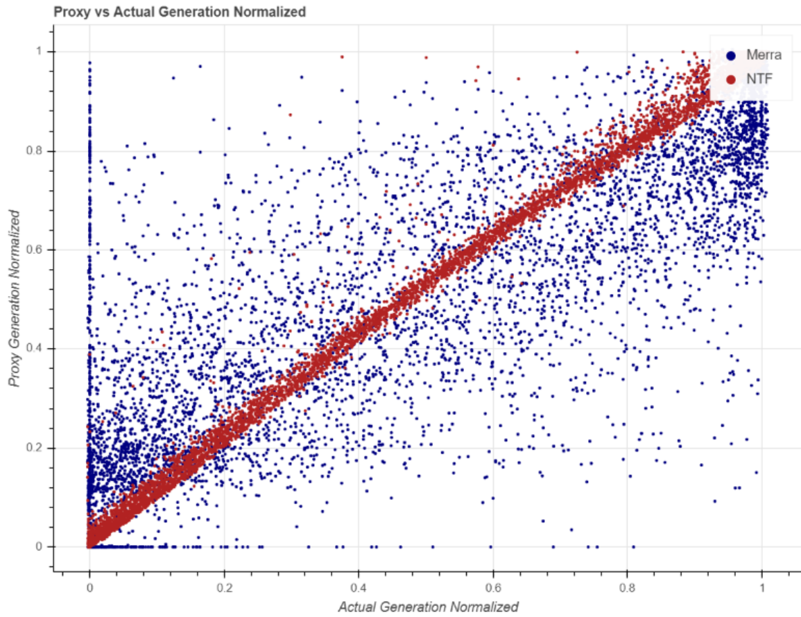
Figure 15: Proxy vs Actual Generation Scatter
