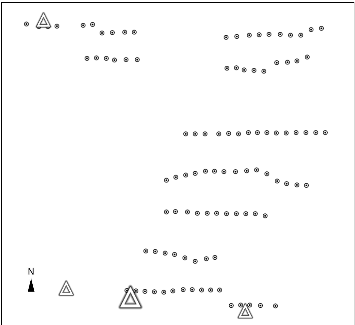
Figure 6: Turbine layout at project
