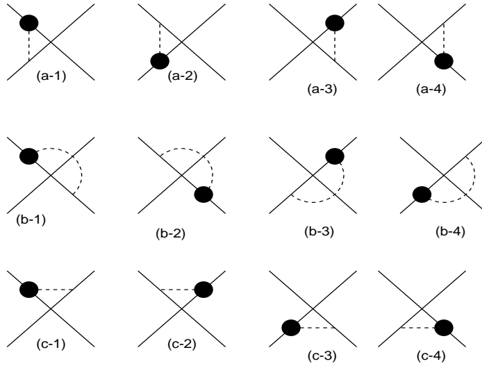
Figure 7: Possible PV chiral corrections to PC NN couplings C_{S,T} .
