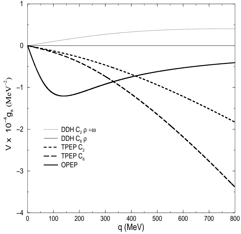
Figure 11: Components of the PV NN potential (in units of g_\pi 10^{-4} \text{MeV}^{-2} ) as function of the momentum transferred (in MeV): OPE (thick solid line); C_6 component of TPE (long-dash line); \tilde{C}_2 component of TPE (short-dash line); C_6 component of DDH (thin solid line); \tilde{C}_2 component of DDH (dotted line).
