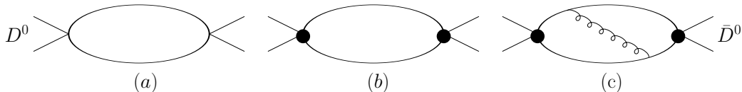
FIG. 1: D^0 \rightarrow \bar{D}^0 : (a) No-QCD, (b) QCD-corrected vertices, (c) an example of NLO correction.
