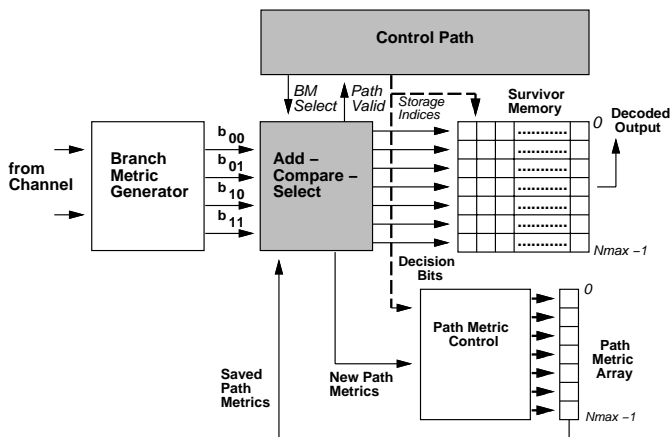
Fig. 1. Adaptive Viterbi decoder architecture
