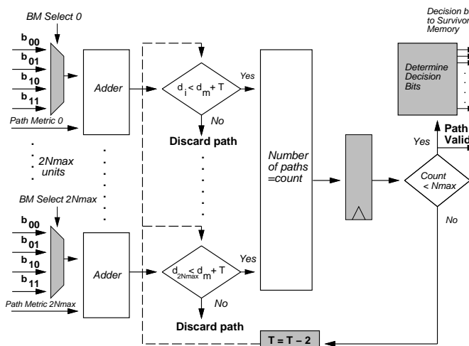
Fig. 2. ACS unit of adaptive Viterbi decoder
