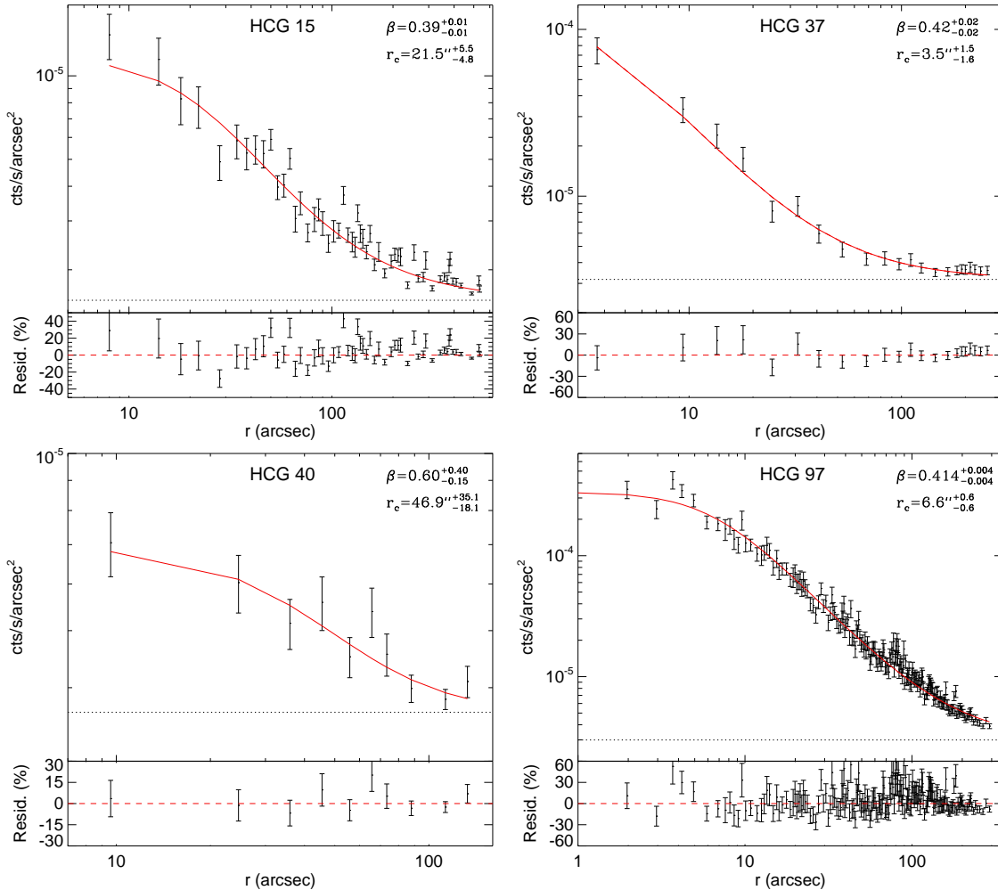
Figure 2. 0.3–2 keV exposure-corrected surface brightness profiles of groups with detectable diffuse emission, along with best-fitting \beta -models (solid lines). Horizontal dotted lines mark the estimated background level in each case. For each plot, the bottom panel shows fit residuals relative to the best-fitting model.
