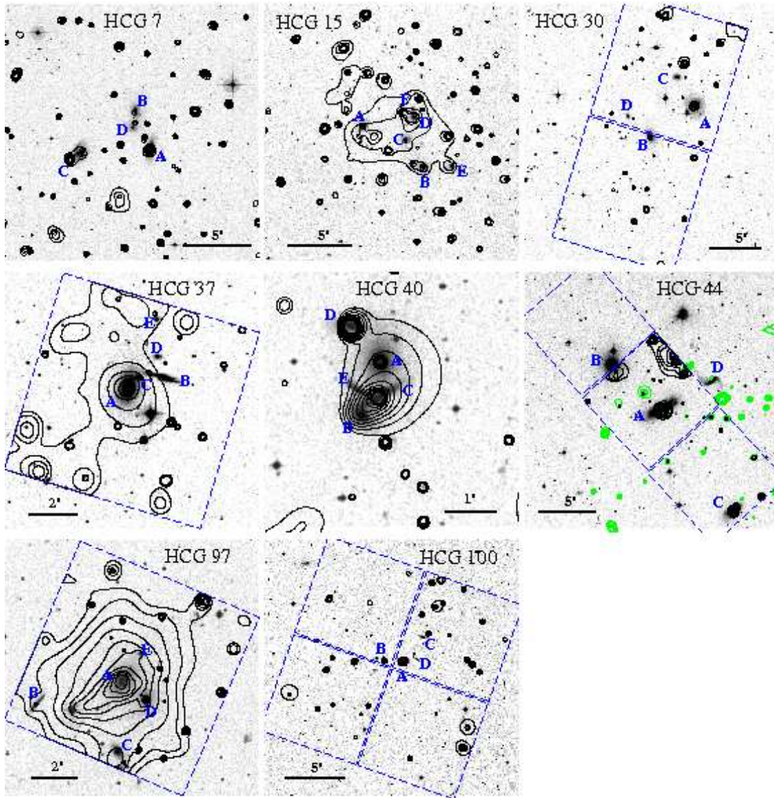
Figure 1. Contours of adaptively smoothed 0.3–2 keV emission overlaid on DSS images for all groups, with the principal group members labelled following the notation of Hickson (1982). Where relevant, dashed squares outline the coverage of the Chandra /ACIS CCD’s. For HCG 44, dark (black) contours outline the Chandra emission, and lighter (green) those of an overlapping XMM pointing.
