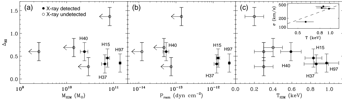
Figure 5. HI deficiency and (a) hot gas mass inside the region used for determining \Delta_{\text{HI}} , (b) characteristic ram pressure, and (c) hot gas temperature for the various groups. Empty circles represent groups with no detectable hot gas. Inset in (c) shows velocity dispersion vs. T_{\text{IGM}} for the X-ray detected groups, with the Osmond & Ponman (2004) relation, i.e. equation (3), overplotted as a dashed line.
