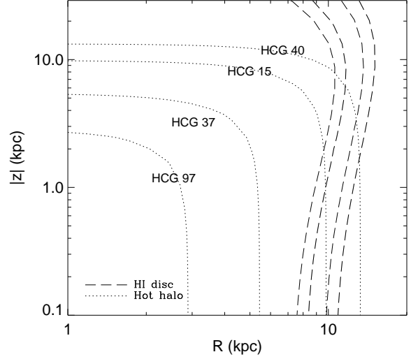
Figure 6. Isobars of gravitational restoring pressure (dashed) and hot halo thermal pressure (dotted) for our fiducial model galaxy in the different groups. Dashed lines outline the galactic regions outside which HI in the disc can be stripped by ram pressure, corresponding to equality in equation (10). Dotted lines show the corresponding regions for the hot halo gas. The order of the contours is the same in both cases.
