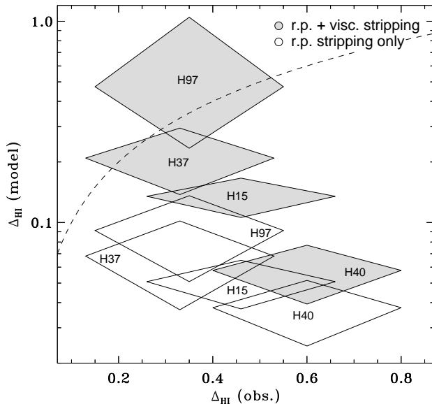
Figure 7. Observed HI deficiencies compared to the model predictions of Table 6 for the stripping of HI by ram pressure alone (empty diamonds), and by ram pressure plus viscous stripping (shaded). Dashed line represents equality between observed and predicted \Delta_{\text{HI}} .
